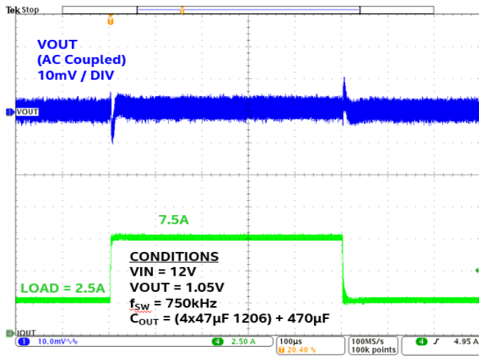
Load Transient 2.5 to 7.5A
