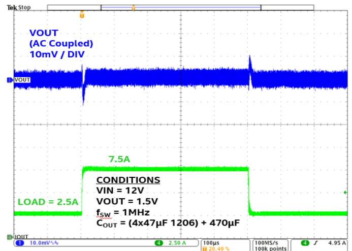
Load Transient 2.5 to 7.5A
