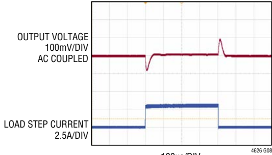
5V Output Transient Response
