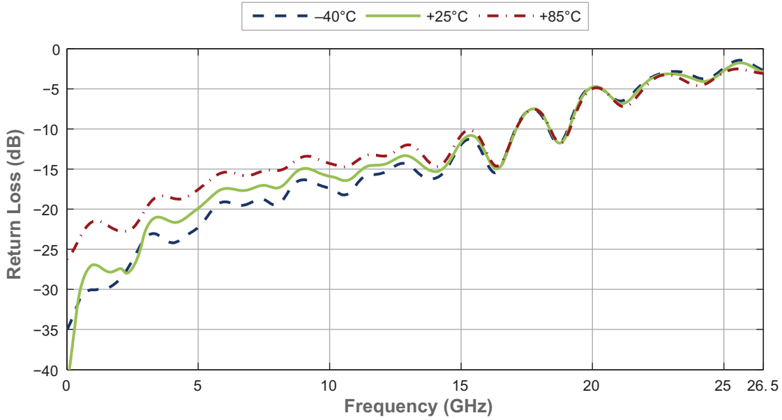
Figure 12 ■ Terminated Port Return Loss vs Temperature
