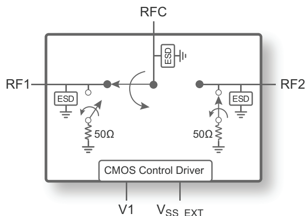
Figure 1 • PE42522 Functional Diagram
