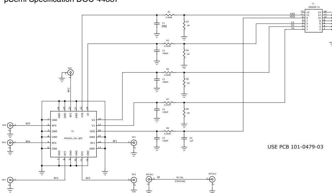
Figure 5. Evaluation Board Schematic pSemi Specification DOC-44837
