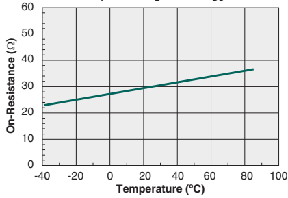
1-Form-B Typical On-Resistance vs. Temperature ( I_F=5\text{mA} , I_L=100\text{mA}_{DC} )
