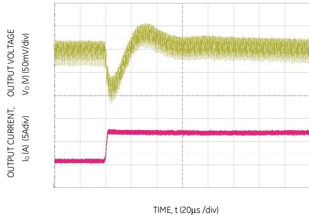
Figure 34. Transient Response to Dynamic Load Change from 50% to 100% at 12Vin, C out = 1x47μF+1x330μF, CTune=2200pF & RTune=300Ω
