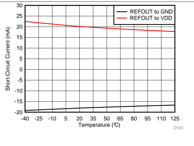
Figure 56. Reference Short-Circuit Current vs Temperature
