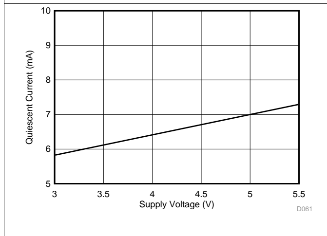
Figure 57. Quiescent Current vs Supply Voltage
