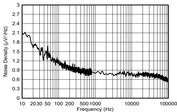
Internal reference, gain = 4x Figure 6-26. Voltage Output Noise Density
