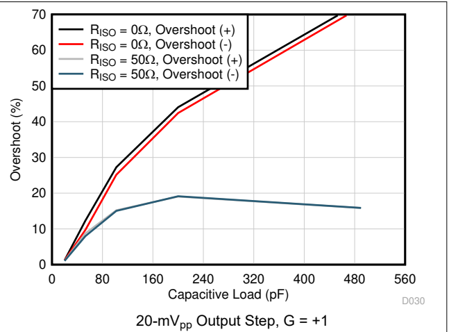
Figure 6-32. Small-Signal Overshoot vs Capacitive Load
