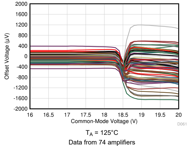
Figure 6-8. Offset Voltage vs Common-Mode Voltage (Transition Region)
