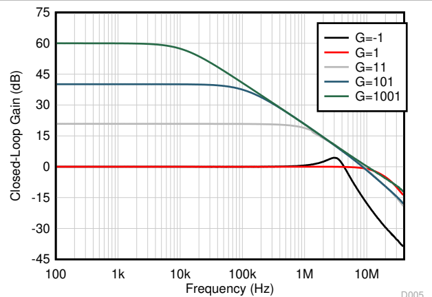
Figure 6-12. Closed-Loop Gain vs Frequency
