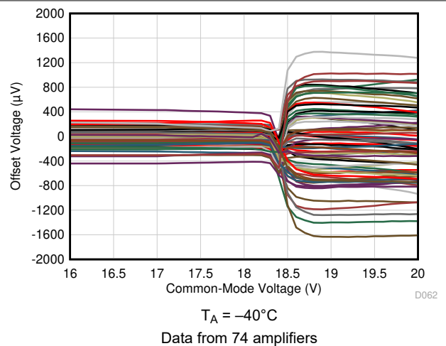
Figure 6-10. Offset Voltage vs Common-Mode Voltage (Transition Region)
