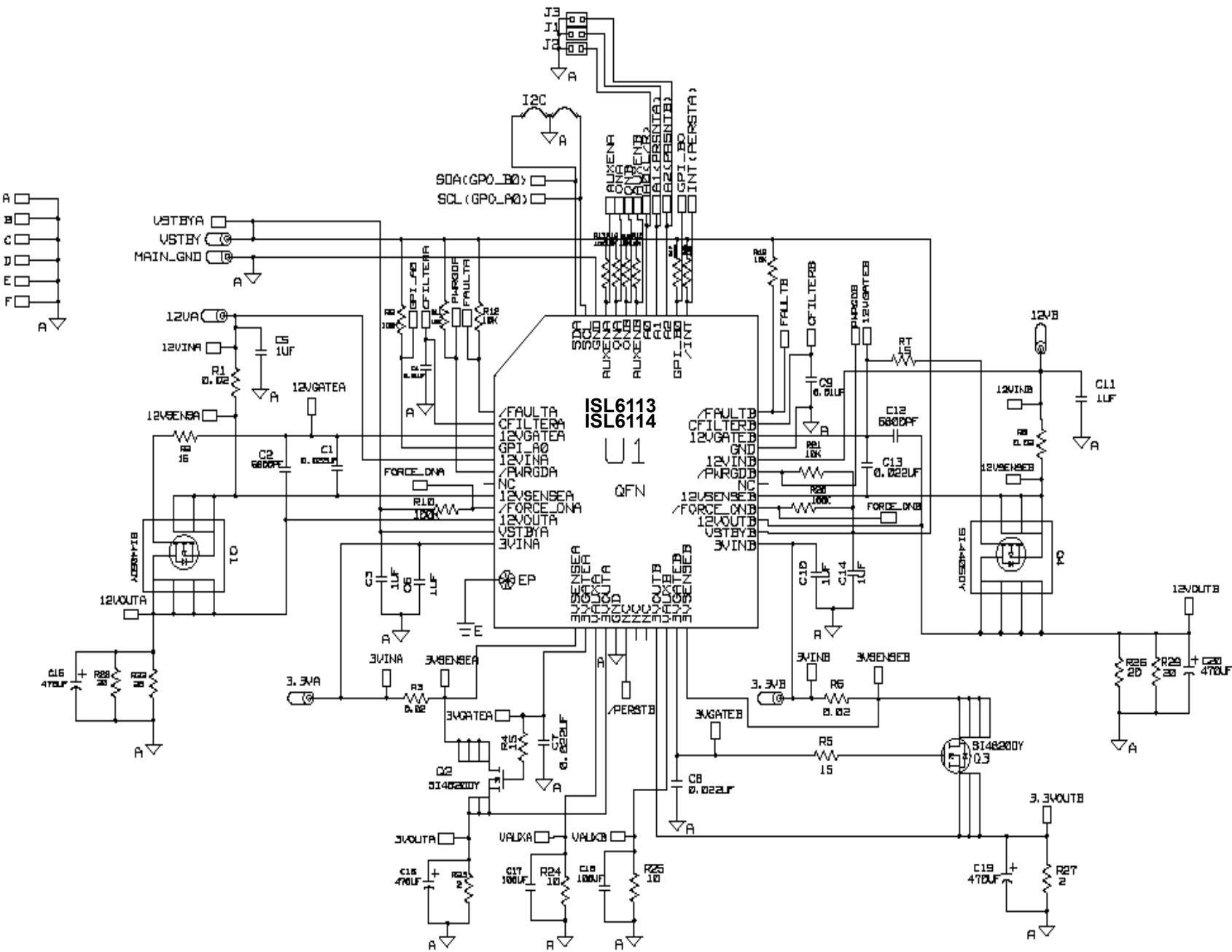
FIGURE 38. ISL6113EVAL1Z, ISL6114EVAL1Z BOARD SCHEMATIC
