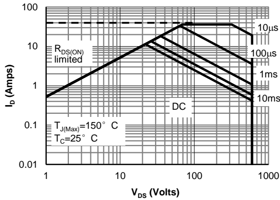
Figure 9: Maximum Forward Biased Safe Operating Area for AOT10N60/AOB10N60 (Note E)
