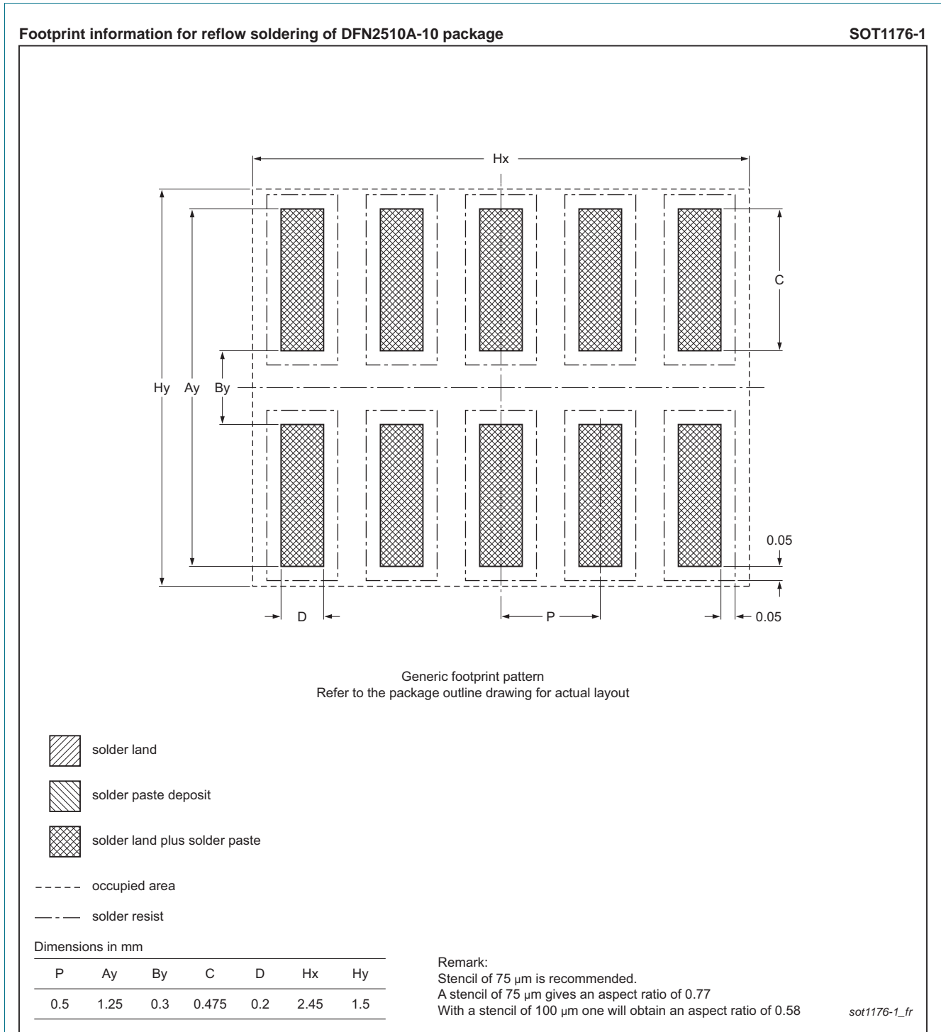
Fig 11. Reflow soldering footprint DFN2510A-10 (SOT1176-1)
