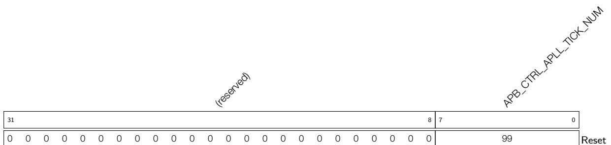
Register 3.5. APB_CTRL_APLL_TICK_CONF_REG (0x003C)
