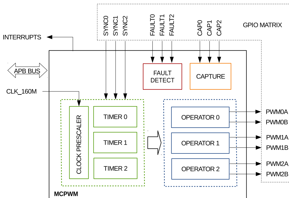
Figure 16-1. MCPWM Module Overview
