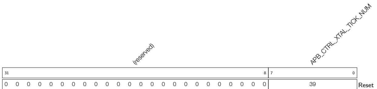
Register 3.2. APB_CTRL_XTAL_TICK_CONF_REG (0x0004)
