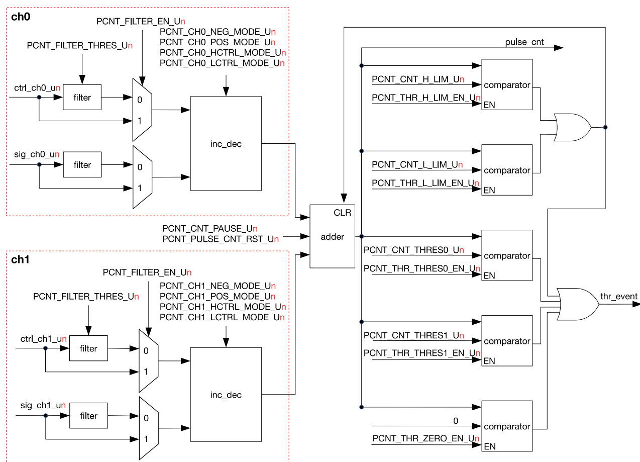
Figure 17-1. PULSE_CNT Architecture
