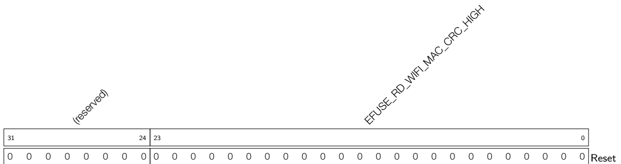
Register 20.3. EFUSE_BLK0_RDATA2_REG (0x008)
