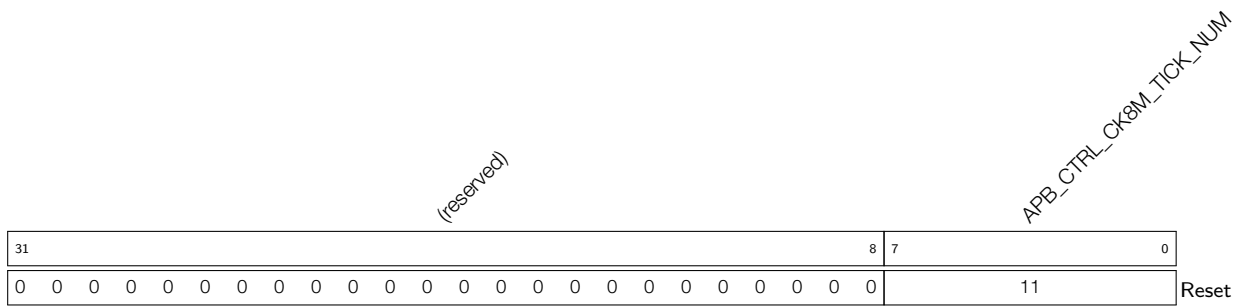
Register 3.4. APB_CTRL_CK8M_TICK_CONF_REG (0x000C)
