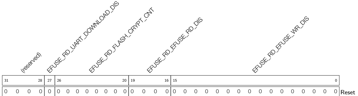
Register 20.1. EFUSE_BLK0_RDATA0_REG (0x000)
