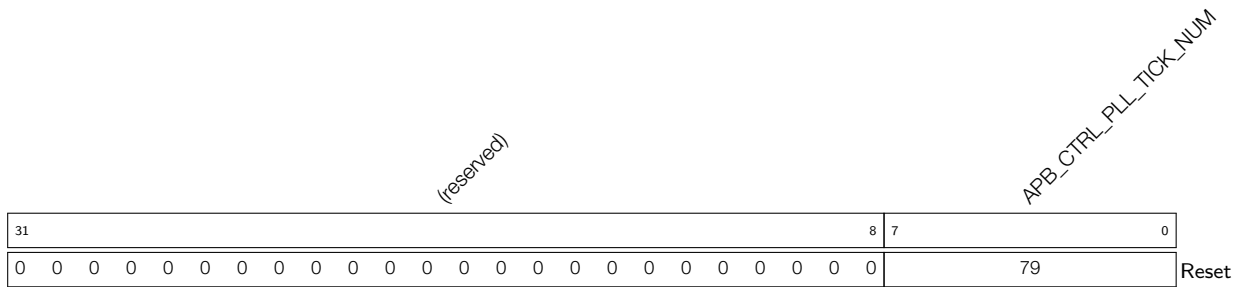
Register 3.3. APB_CTRL_PLL_TICK_CONF_REG (0x0008)
