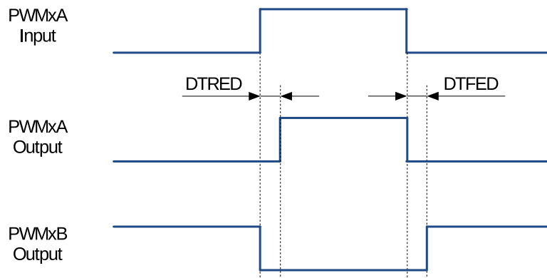
Figure 16-23. Active High Complementary (AHC) Dead Time Waveforms
