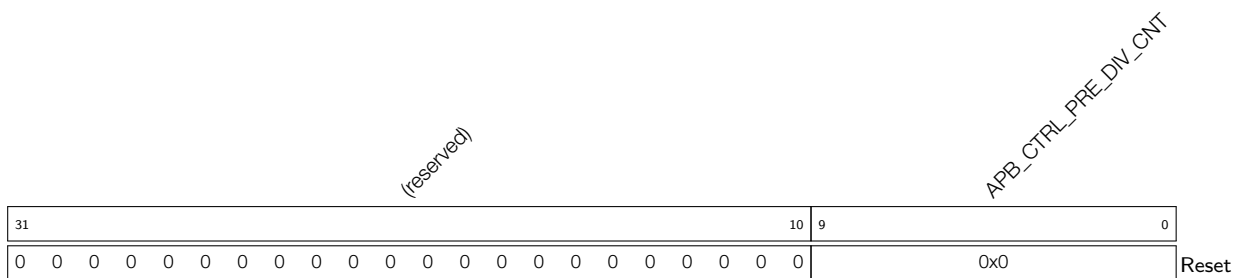
Register 3.1. APB_CTRL_SYSCLK_CONF_REG (0x0000)
