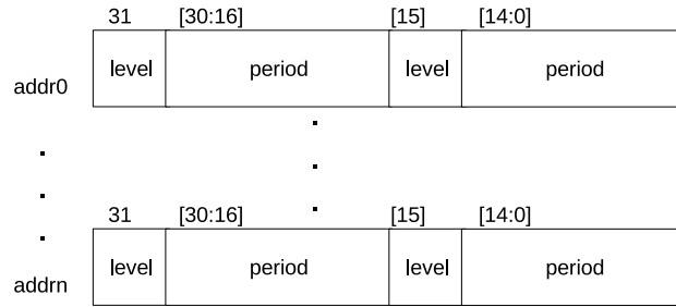
Figure 15-2. Data Structure
