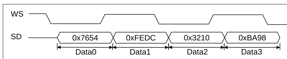
Figure 12-7. The First Stage of Receiving Data
