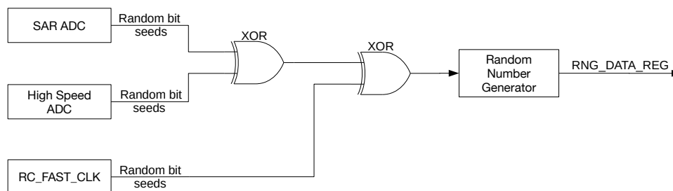
Figure 25-1. Noise Source
