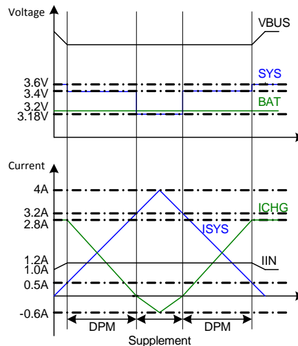
Figure 9. DPM Response
