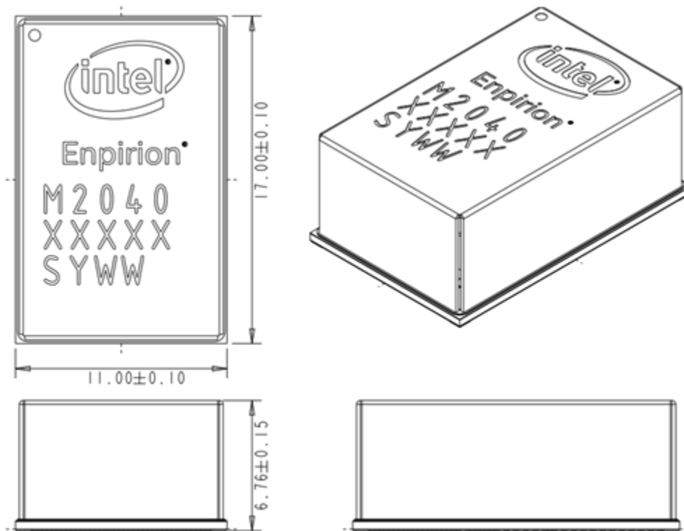
Figure 20: Package Dimensions
