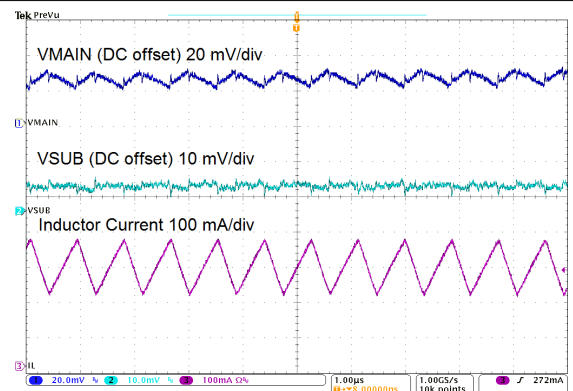
TPS610981 I_{(MAIN)} = 0 \text{ mA} I_{(SUB)} = 100 \text{ mA} MODE = H V_{IN} = 1.5 \text{ V}
