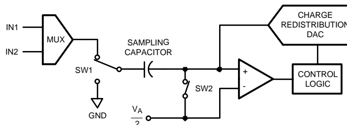
Figure 48. ADC082S051 in Track Mode
