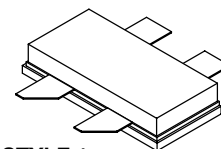
CASE 465H-02, STYLE 1 NI-780S-4 MRF8P23080HSR3
