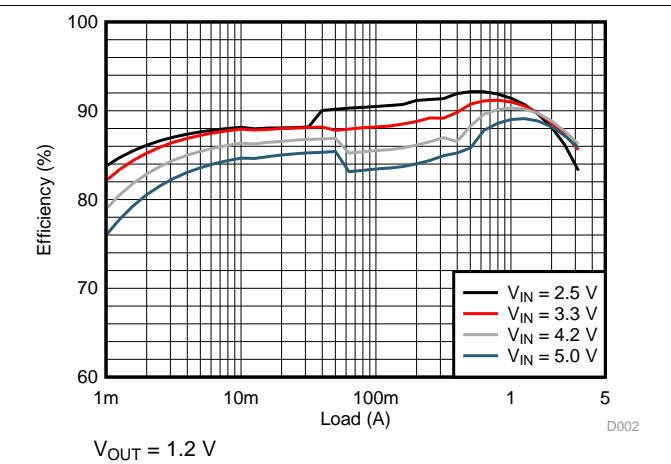
Figure 6. Efficiency
