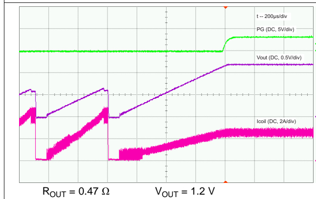
Figure 21. Output Short-Circuit Protection, Recovery
