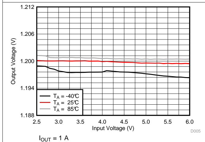
Figure 9. Line Regulation
