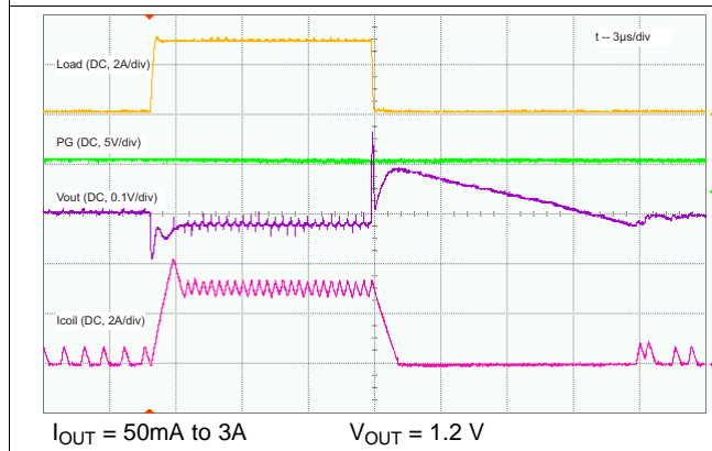
Figure 19. Load Transient
