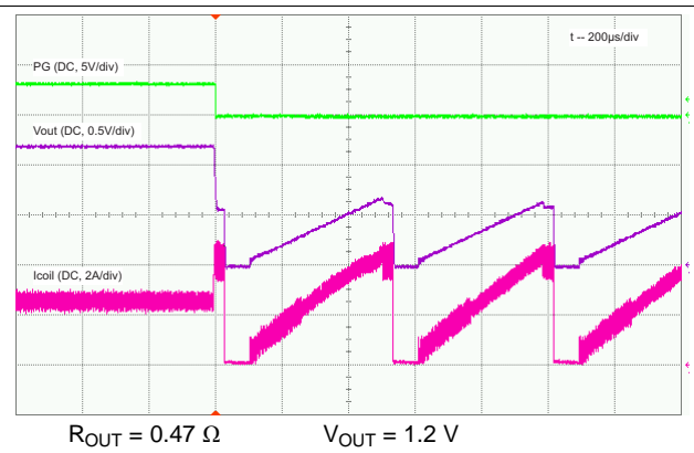
Figure 20. Output Short-Circuit Protection, Entry
