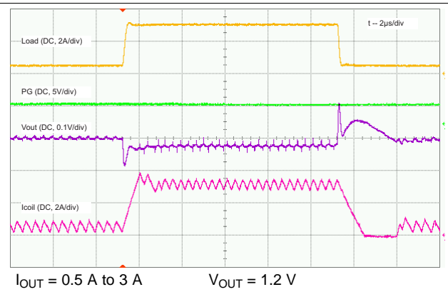
Figure 18. Load Transient
