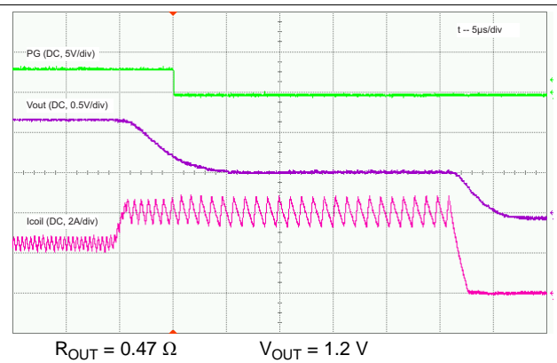
Figure 22. Output Short-Circuit Protection, HICCUP Zoom In
