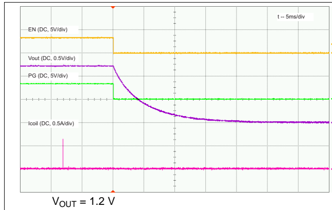
Figure 17. Shutdown without Load
