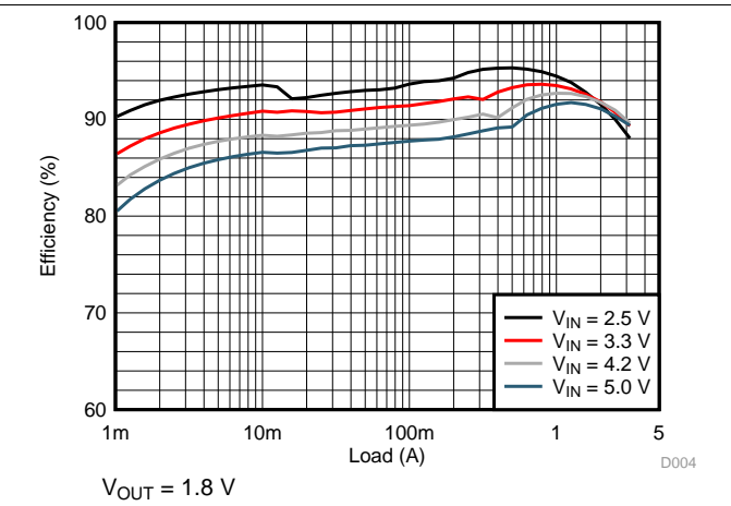
Figure 8. Efficiency
