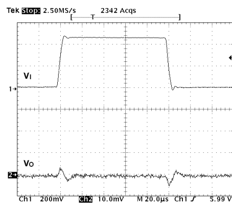
V_I = [V_{O(NOM)} + 1V], V_O = 4.7V, I_O = 100mA, C_O = 4.7\mu F (X7R)
