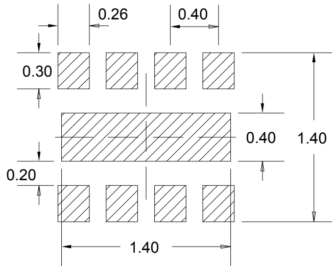
Figure 26. DFN8 (1.6x1.2 mm) recommended footprint
