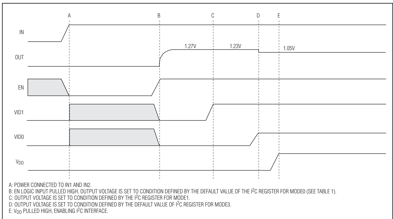
Figure 2. Power-Up Sequence
